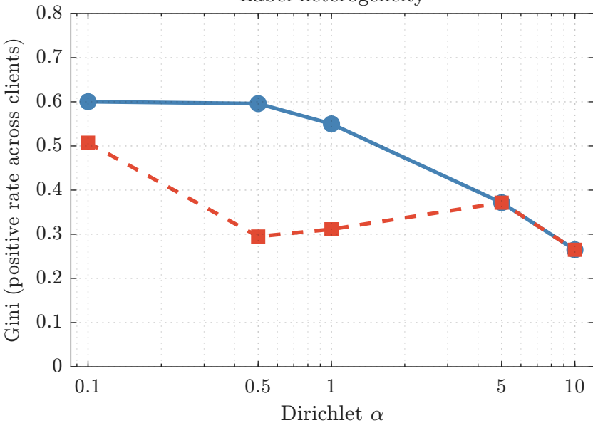
Label heterogeneity
